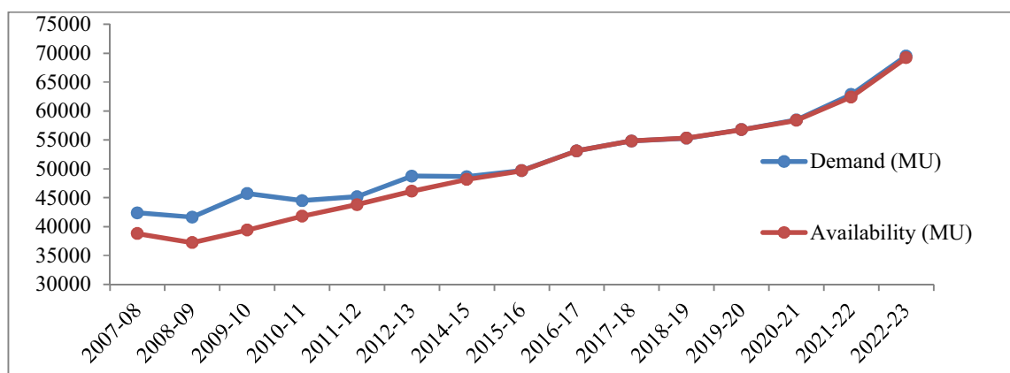
Figure 53: Power requirement and availability in Punjab
